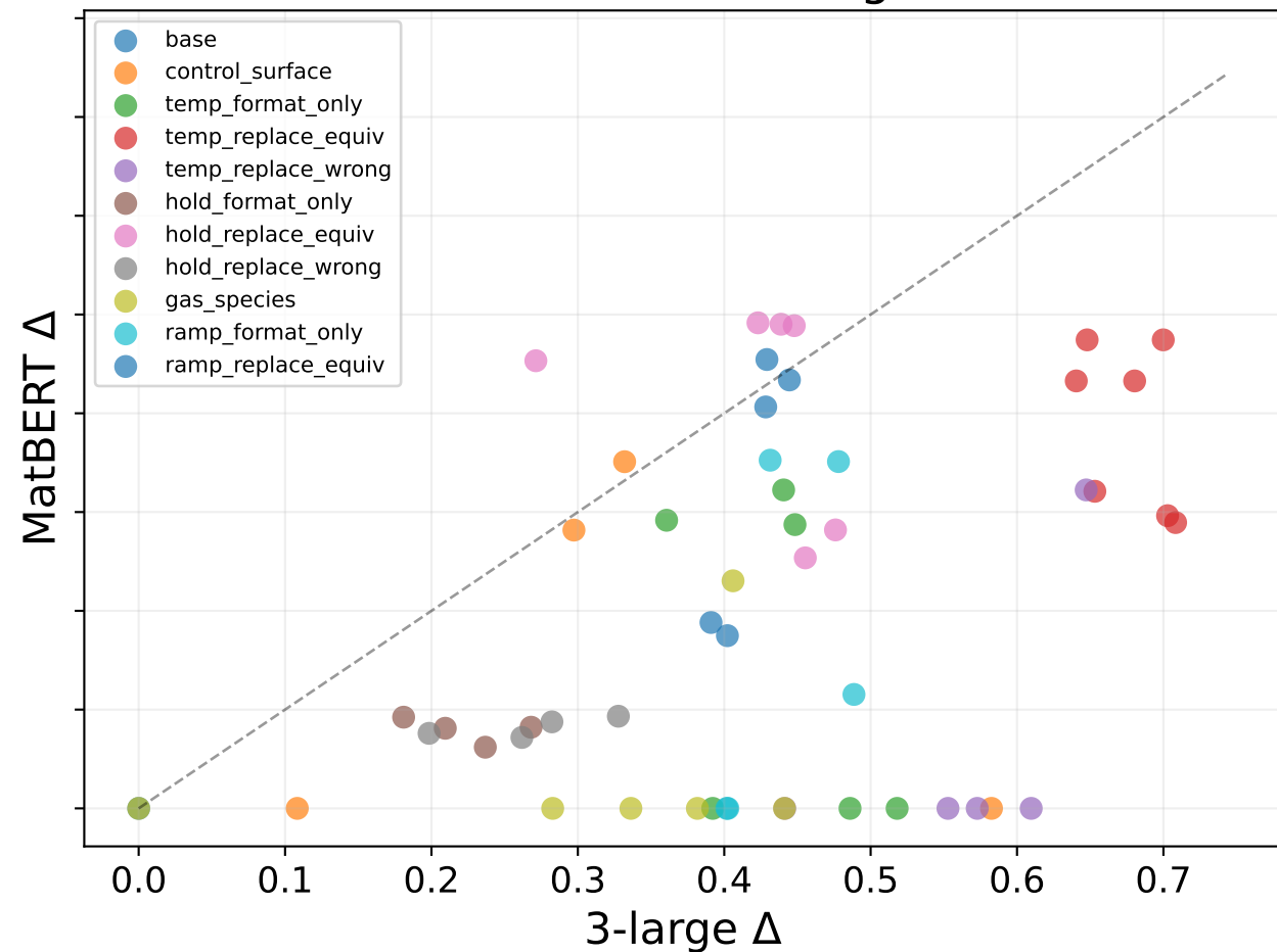
MatBERT vs 3-large
